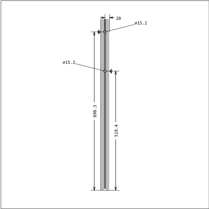
DRAWING 5, Pos 9 SIDE 4
