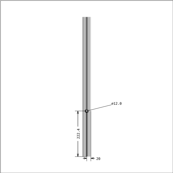
DRAWING 3, Pos 7 SIDE 1, bar length: 681.0 mm
