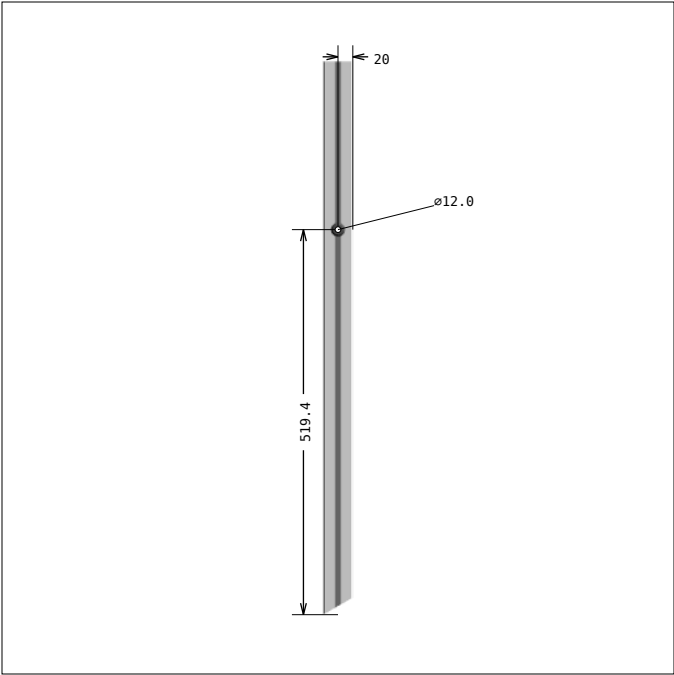
DRAWING 5, Pos 9 SIDE 3
