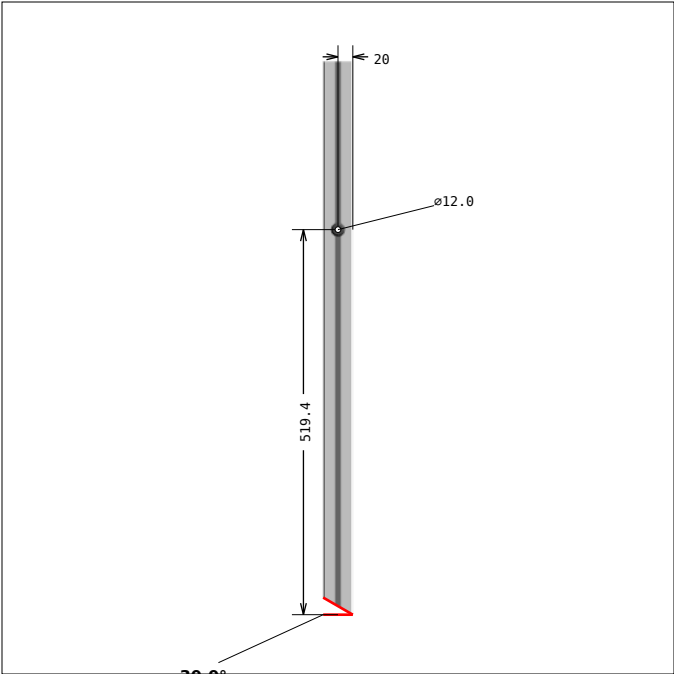
DRAWING 6, Pos 10 SIDE 1, bar length: 746.4 mm
