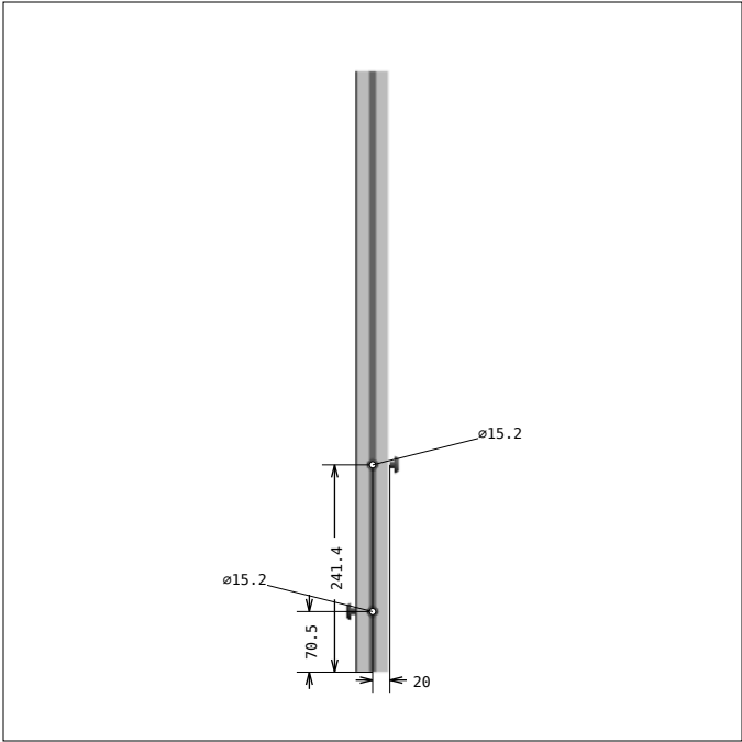
DRAWING 4, Pos 8 SIDE 4
