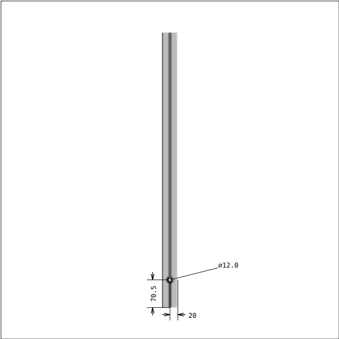
DRAWING 4, Pos 8 SIDE 1, bar length: 700.0 mm
