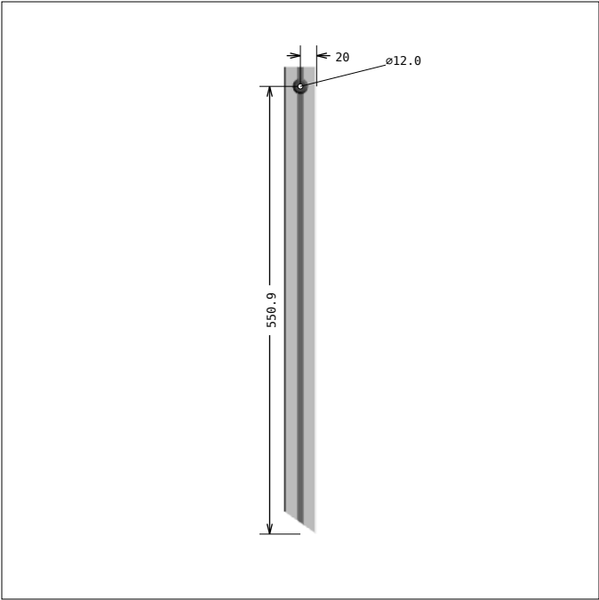
DRAWING 1, Pos 4 SIDE 3
