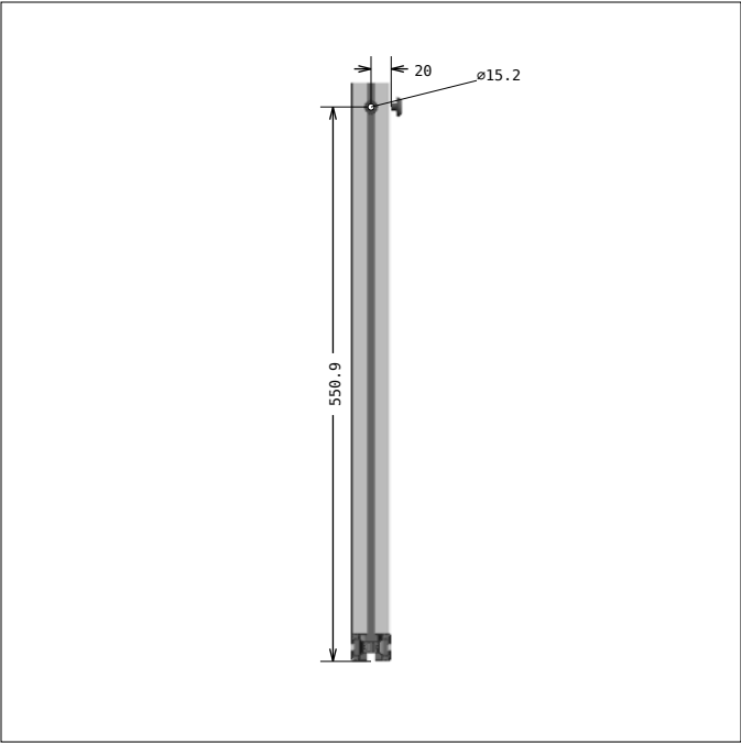
DRAWING 1, Pos 4 SIDE 4
