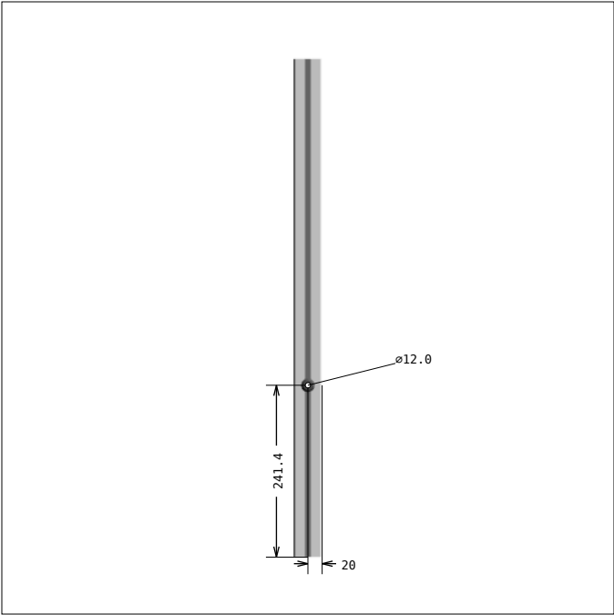
DRAWING 4, Pos 8 SIDE 3
