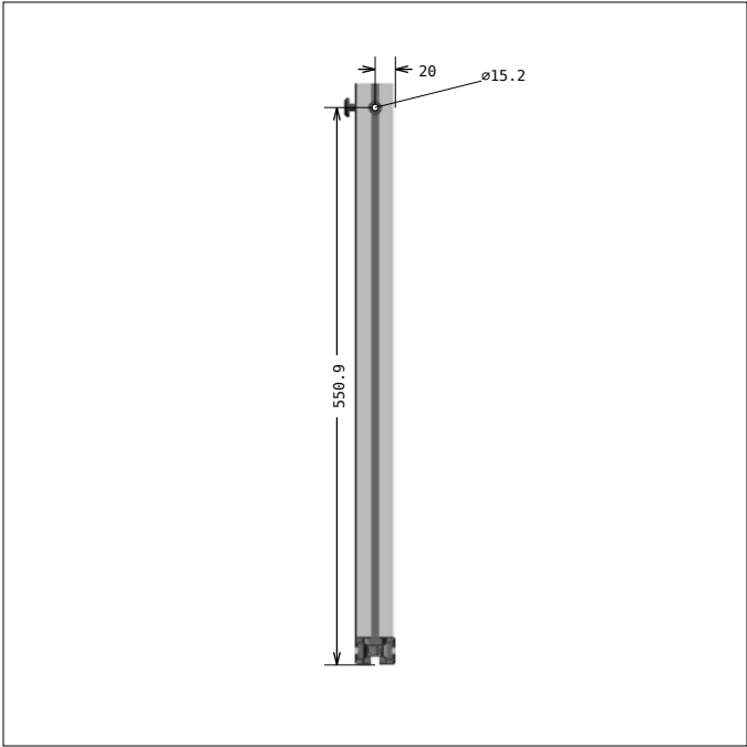
DRAWING 2, Pos 5 SIDE 4
