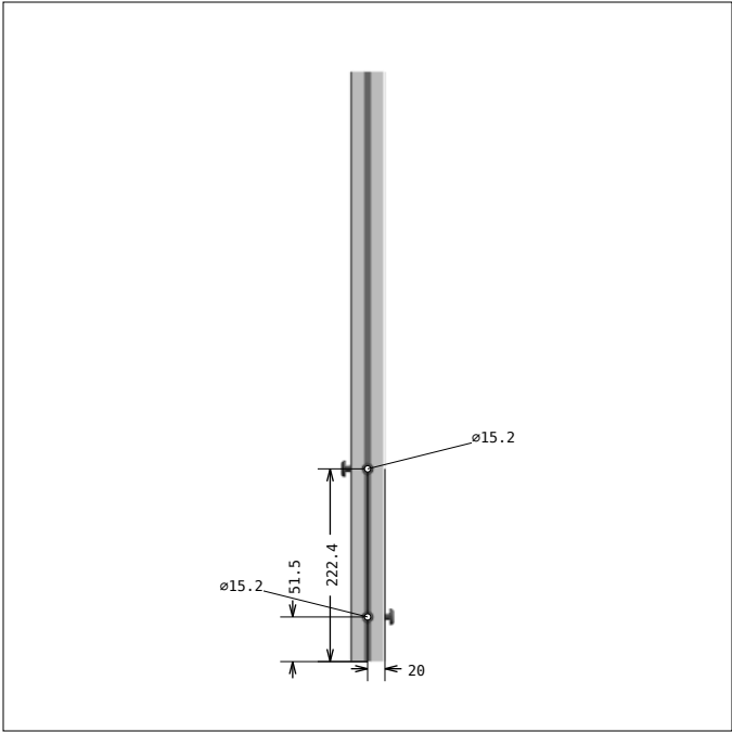
DRAWING 3, Pos 7 SIDE 4
