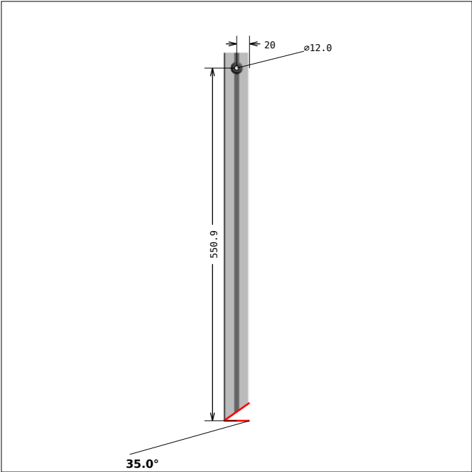
DRAWING 2, Pos 5 SIDE 1, bar length: 575.0 mm
