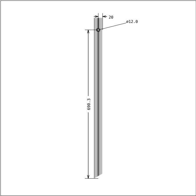
DRAWING 6, Pos 10 SIDE 3
