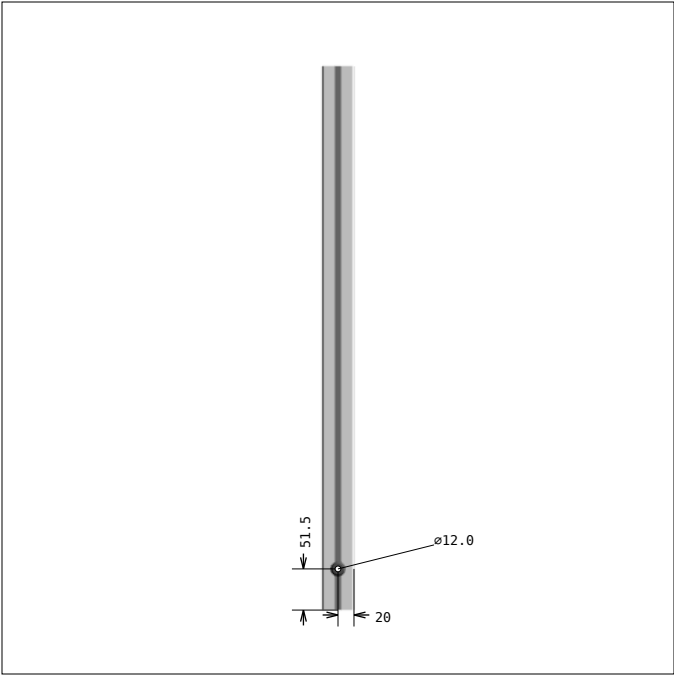
DRAWING 3, Pos 7 SIDE 3
