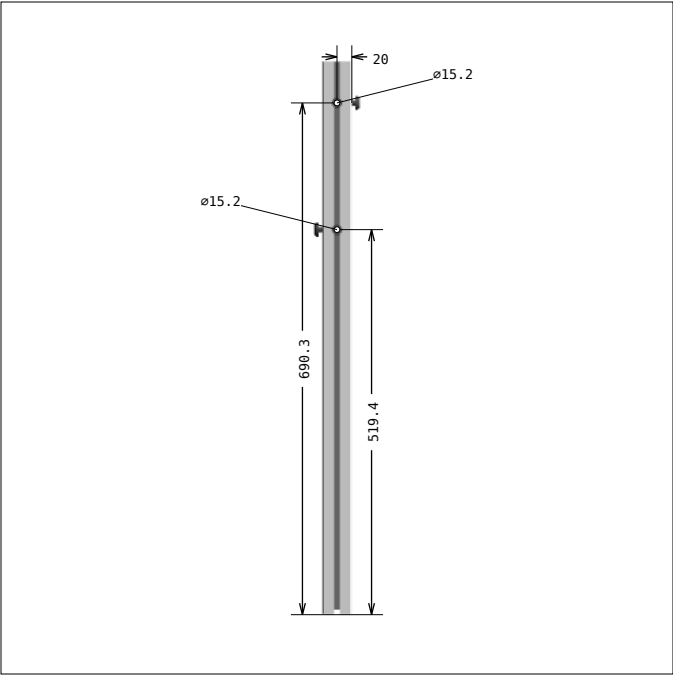
DRAWING 6, Pos 10 SIDE 4
